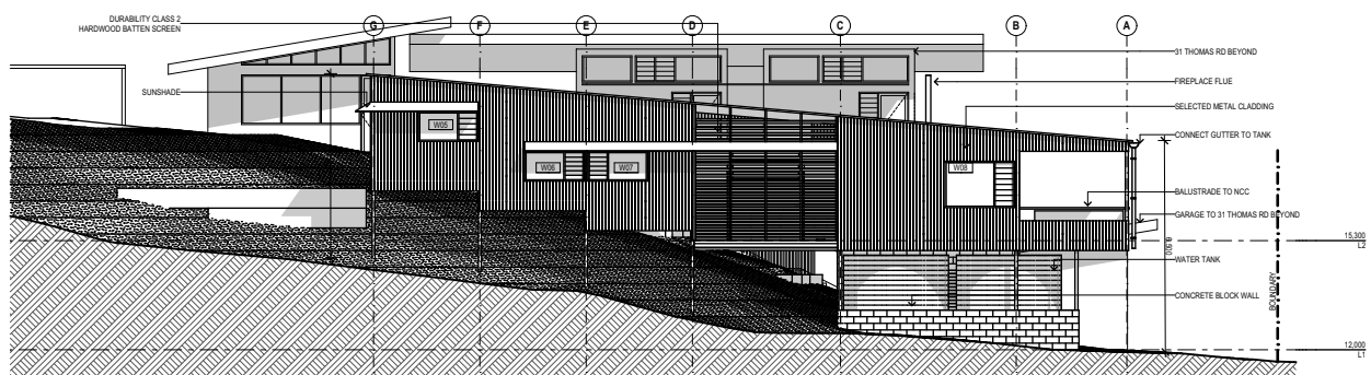
E-03 NORTHEAST 1:250
