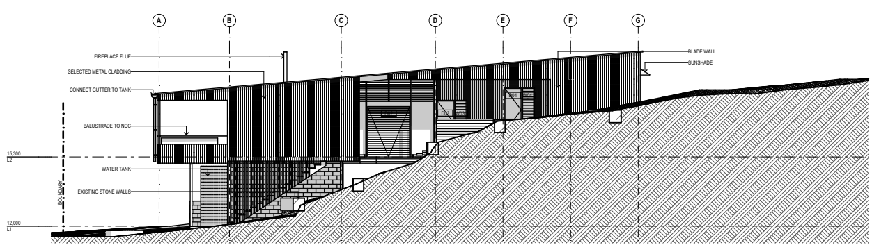
E-01 SOUTHWEST 1:250
