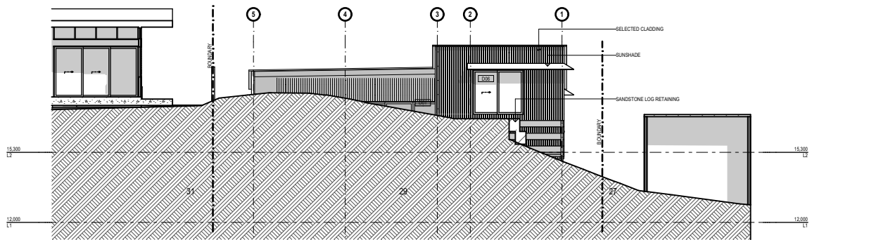
E-02 SOUTHEAST 1:250
